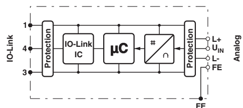
Block diagram
