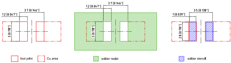
Component Location on Pad
