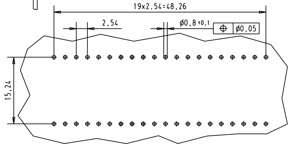
Printed board layout
