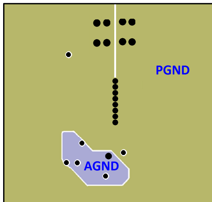
Figure 9: Inner Layer 2 – grounds
