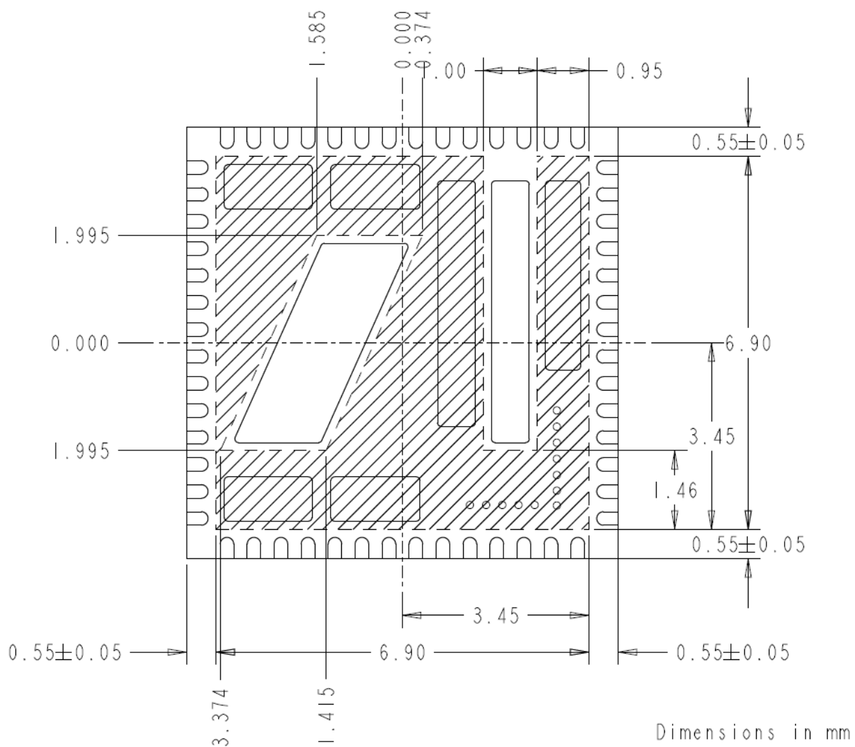
Figure 13: EN6362QI Package – PCB Footprint Keepout (Bottom view)
