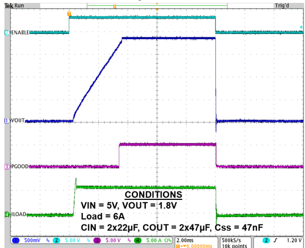
Startup Waveform
