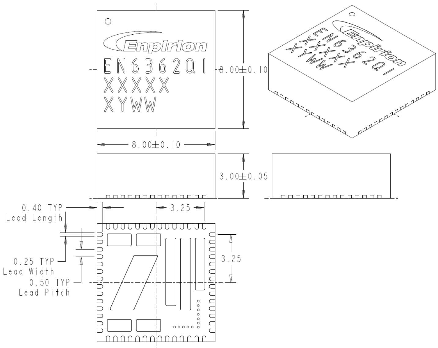
Figure 15: EN6362QI Package Dimensions
