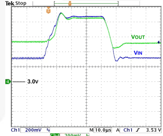
Figure 26. Line Transient, 3.3-3.9 V_{IN} , 10 \mu\text{s} Edge, 500 mA load, V_{OUT}=3.5\text{ V}
